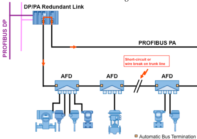
Ring Redundancy on Profibus PA is Possible with Active Field Distributors with Automatic Bus Termination.
